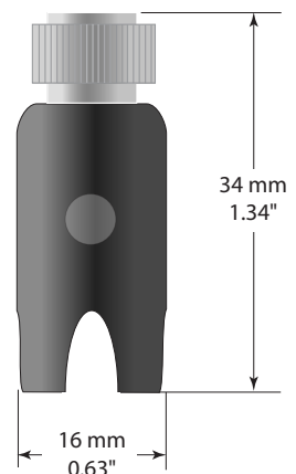
TT-MINI-PROBE dimensions
