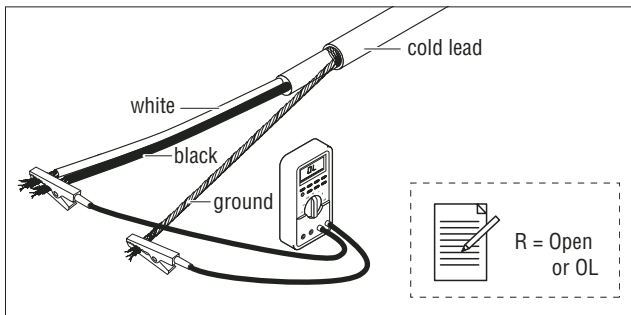
Figure 12: Insulation Resistance test
