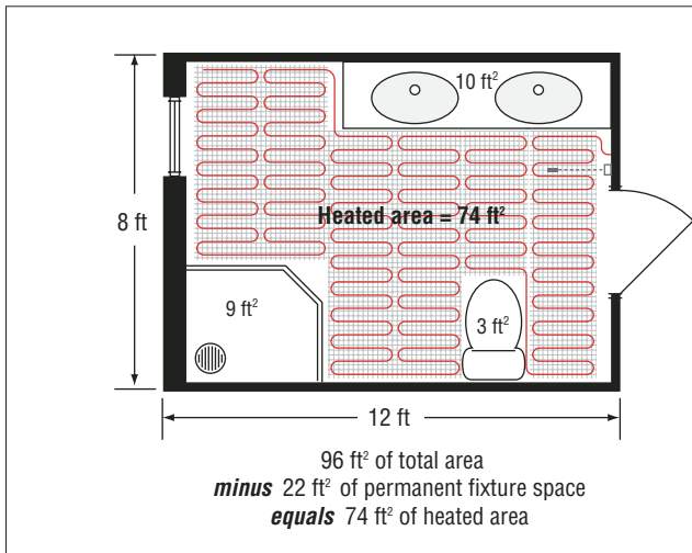
Figure 4: Heated area example
