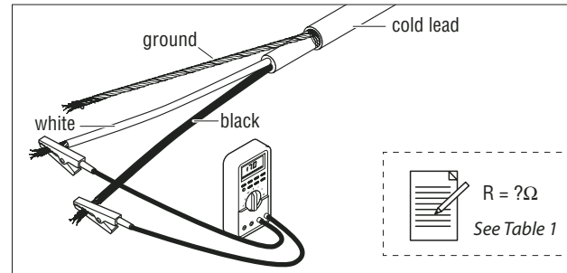
Figure 13: Heating Cable Resistance test
