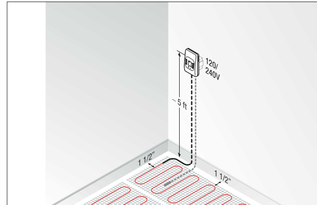
Figure 5: Typical cold lead and floor temperature sensor example
