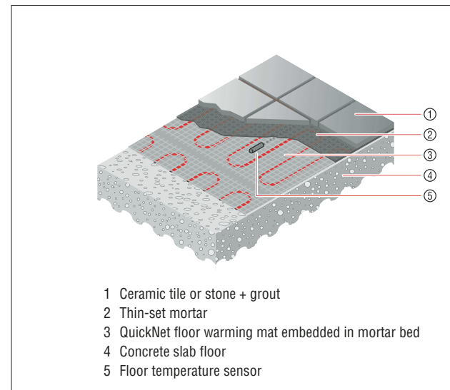
Figure 3: Typical concrete slab
