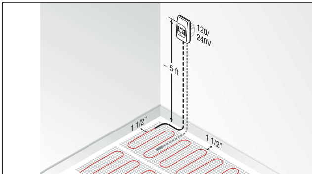
Figure 9: Routing the cold lead
