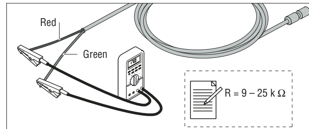
Figure 14: Sensor Resistance test
