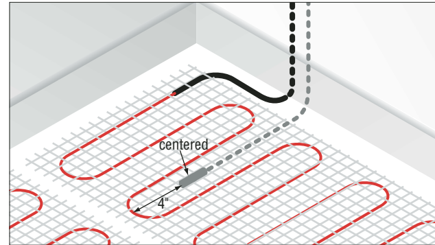
Figure 10: Placing the floor temperature sensor
