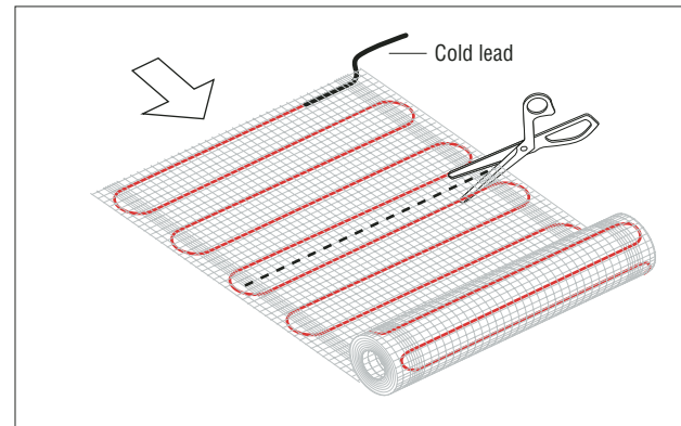
Figure 7: Cutting the mesh
