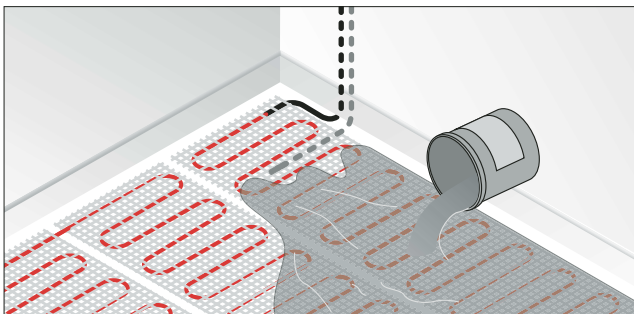
Figure 11: Applying self-leveling mortar
