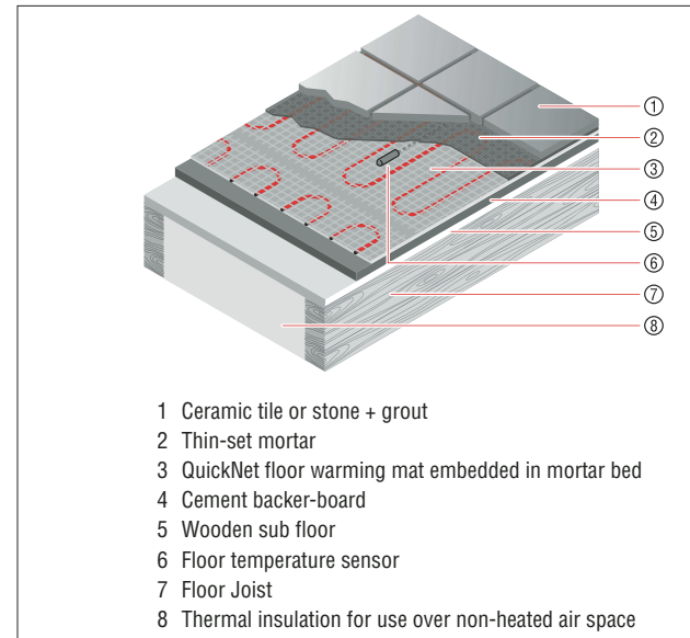
Figure 2: Typical wooden sub floor
