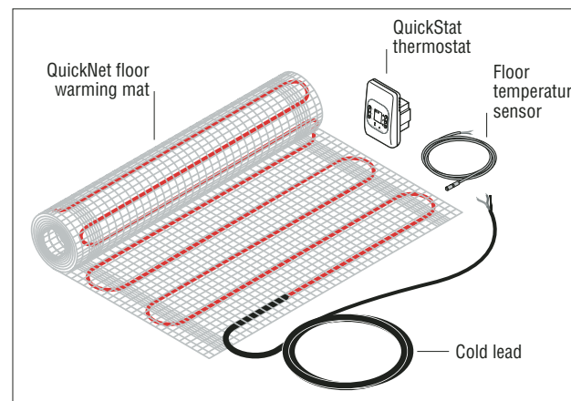
Figure 1: QuickNet system components
