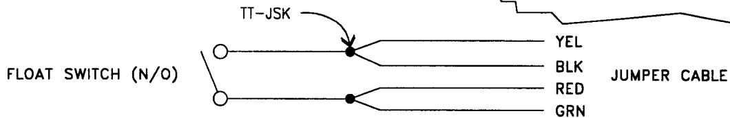
WIRING DIAGRAM
